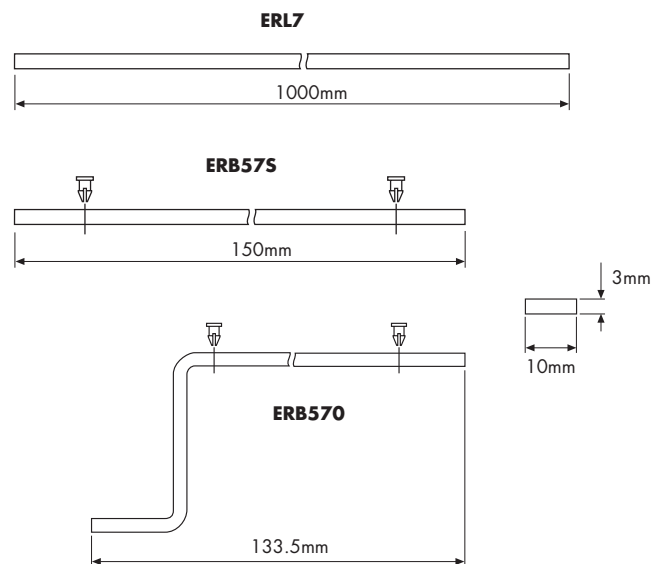
Figure 4.4: Mounting details
