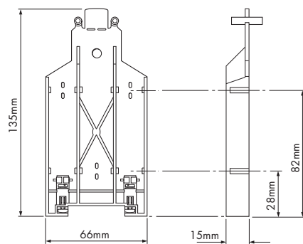
Figure 4.5: IMB57 Insulating mounting block
