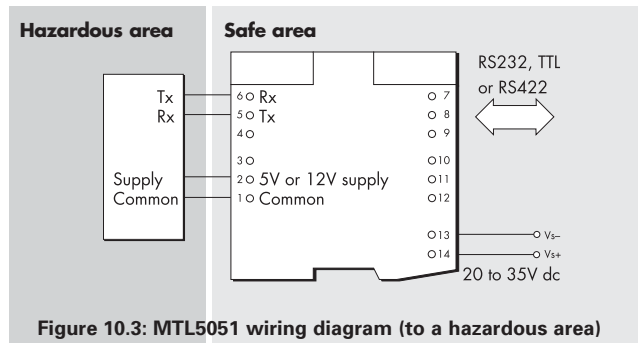
Figure 10.3: MTL5051 wiring diagram (to a hazardous area)
