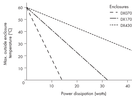
Figure 5.1: Graph depicting outside enclosure temperature limits for DX enclosures used with MTL5500 isolators
