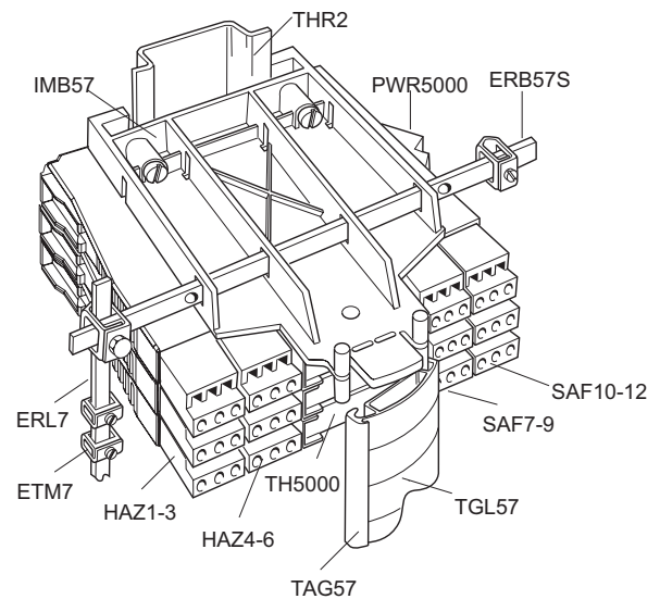
Figure 4.4: Mounting details
