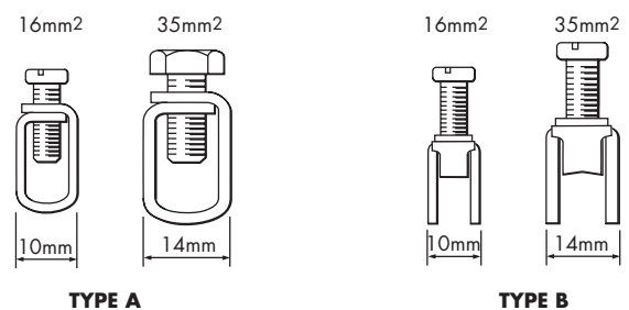
Figure 4.9: Earth rails and clamps
