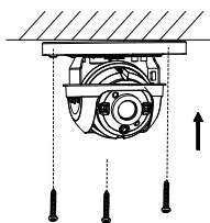
Figure 2-13 Install the Mounting Base
