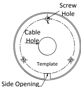
Figure 2-1 Drill Template
