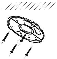
Figure 2-10 Secure the Adapter Plate
