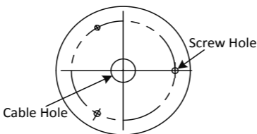
Figure 2. 8 Drill Template
