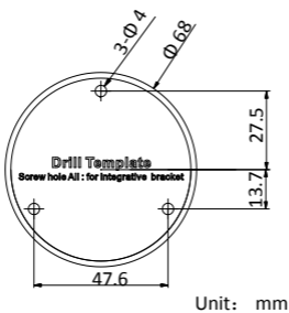
Figure 2. 1 Drill Template
