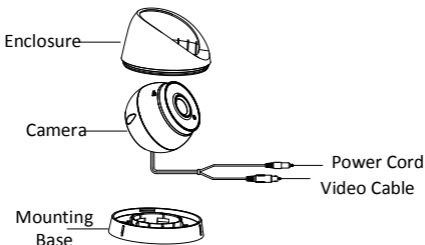
Figure 1. 3 Type III Camera Overview
