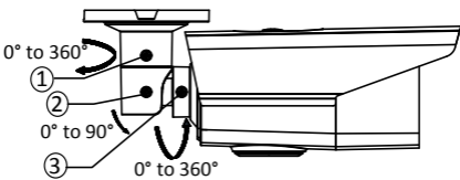
Figure 2. 3 3-Axis Adjustment
