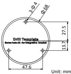
Figure 2. 4 Drill Template
