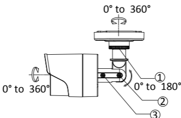
Figure 2. 6 3-Axis Adjustment
