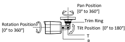
Figure 2-2 3-Axis Adjustment
