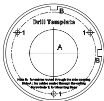
Figure 2-3 Drill Template for Junction Box
