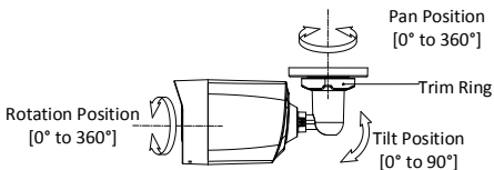
Figure 2-8 3-Axis Adjustment
