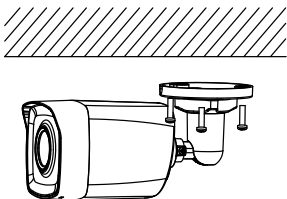
Figure 2-7 Secure the Camera on the Ceiling
