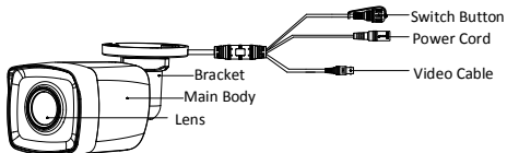
Figure 1-5 Overview of Type III Camera (with F)
