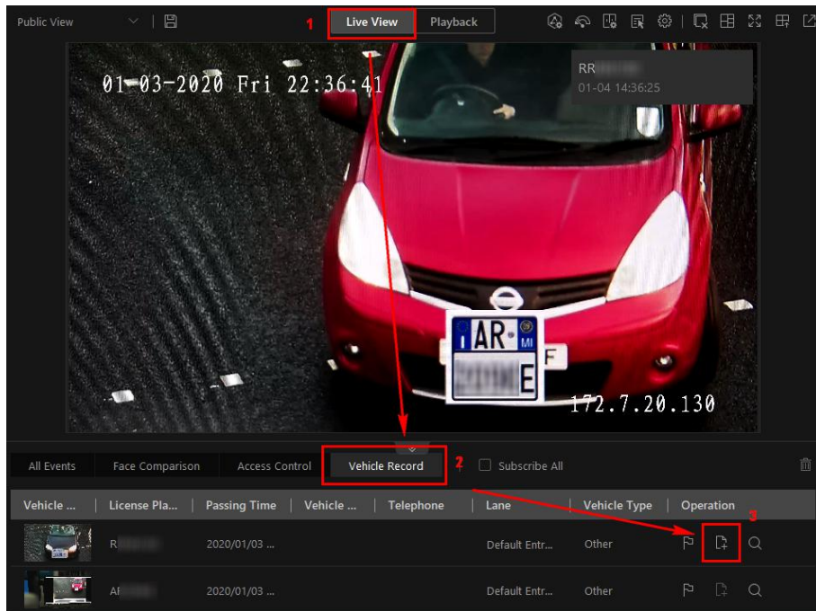
Figure 14-17 Recognized Vehicles
