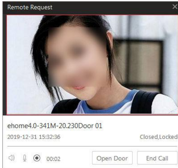
Figure 13-3 Answer Call
