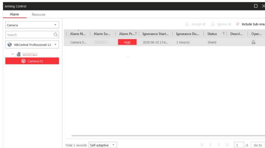
Figure 17-1 Arming Control
