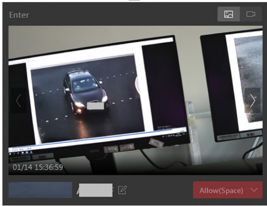
Figure 14-4 Vehicle Entering
