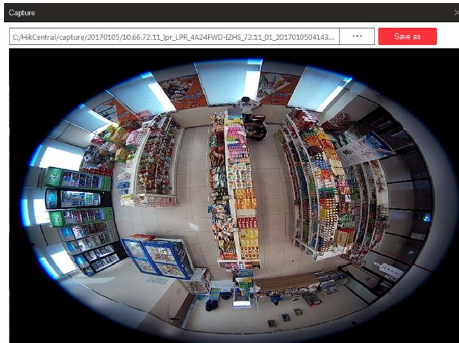
Figure 5-5 Snapshot Window
