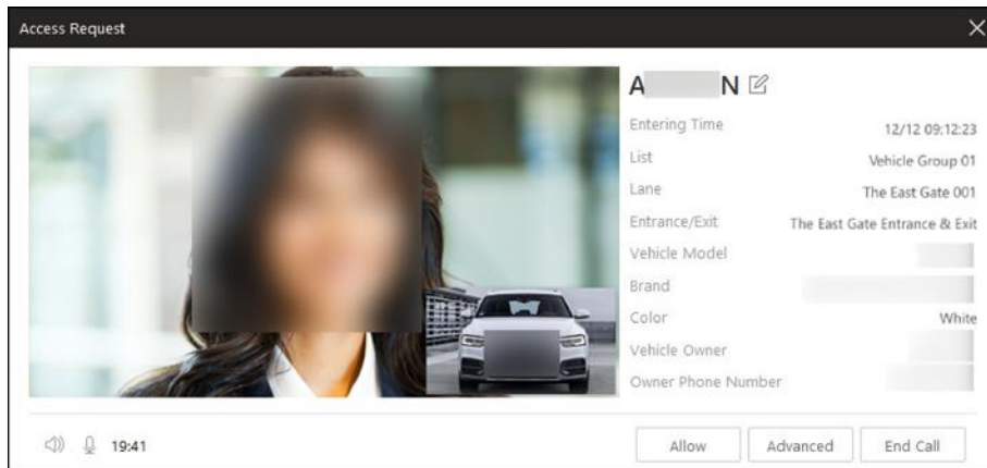
Figure 14-14 Video Intercom
