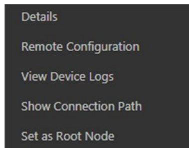
Figure 21-10 More Functions
