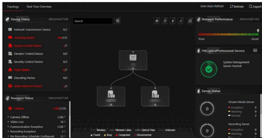
Figure 21-3 Topology
