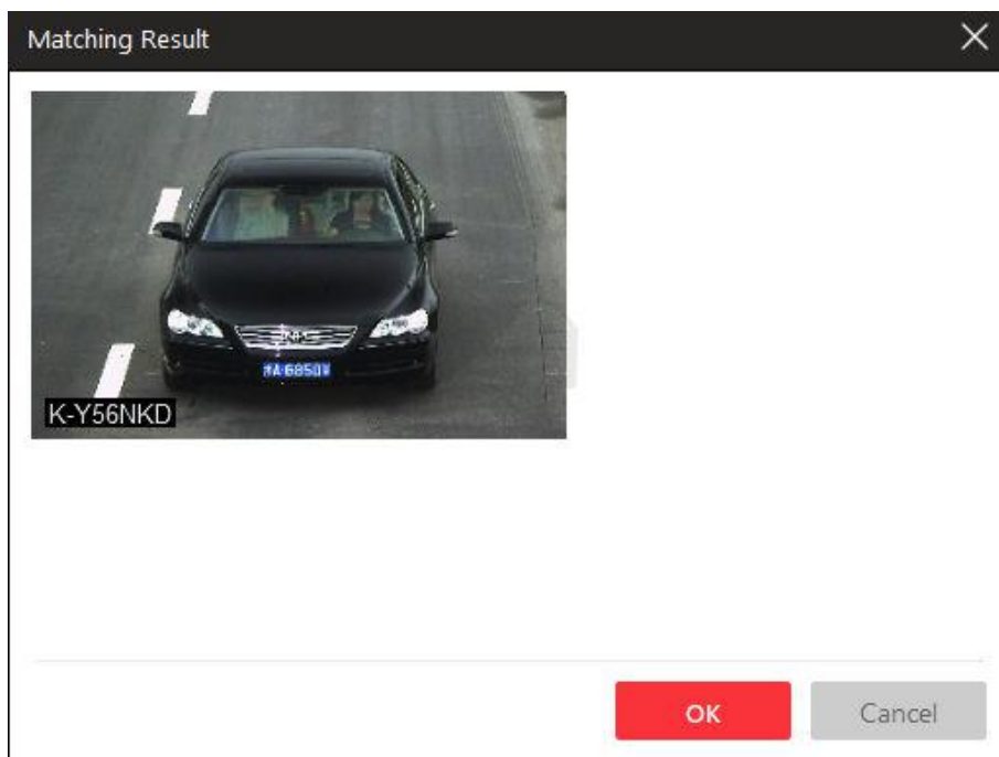
Figure 14-6 Matching Result
