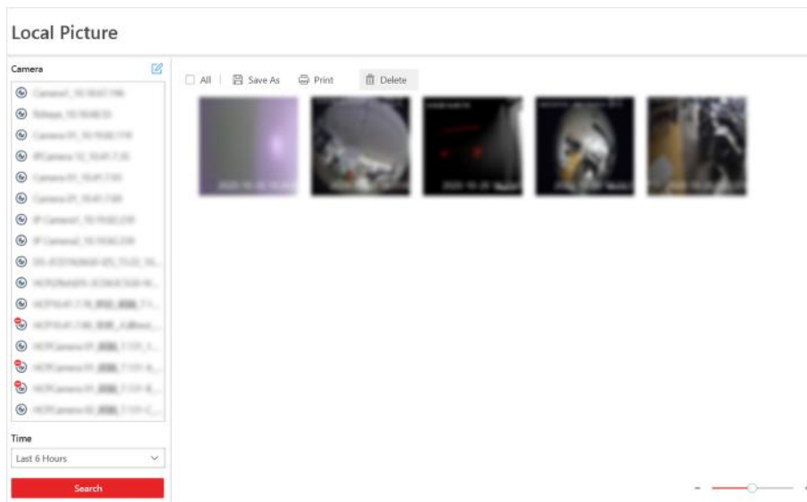
Figure 5-7 Local Picture
