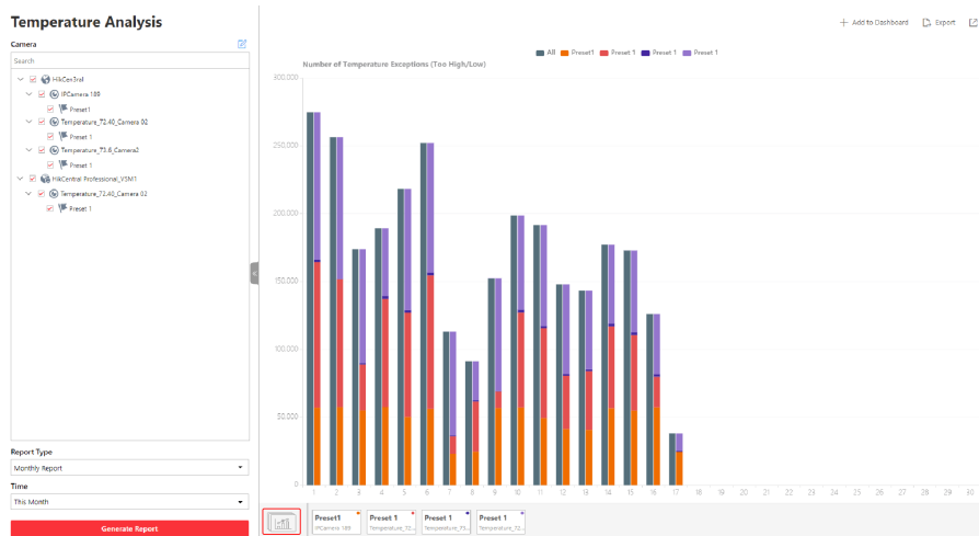
Figure 20-12 Temperature Report
