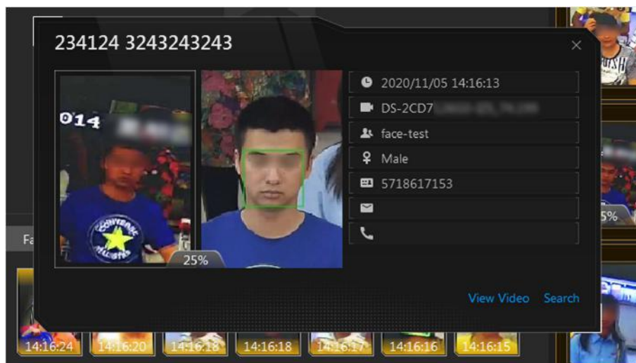
Figure 15-2 Matched Persons
