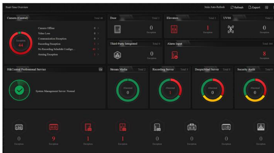
Figure 21-1 Real-Time Overview
