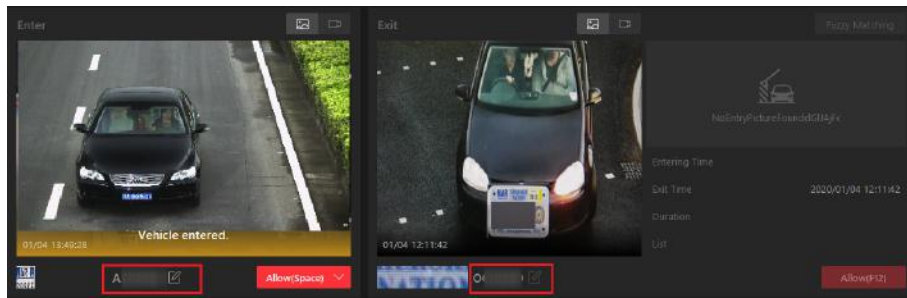
Figure 14-15 Entrance/Exit Page
