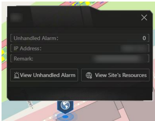
Figure 11-1 Site Details
