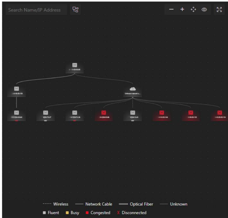
Figure 21-5 Topology Overview
