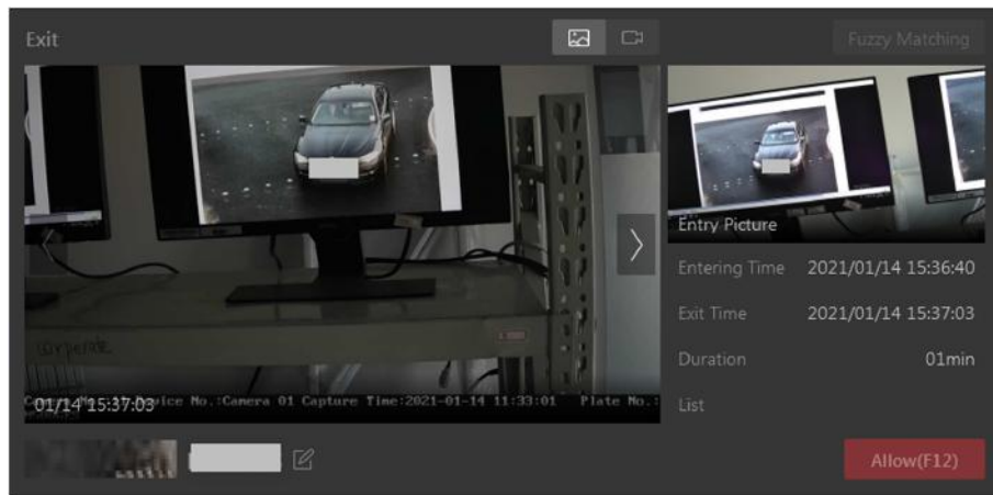
Figure 14-5 Vehicle Exiting
