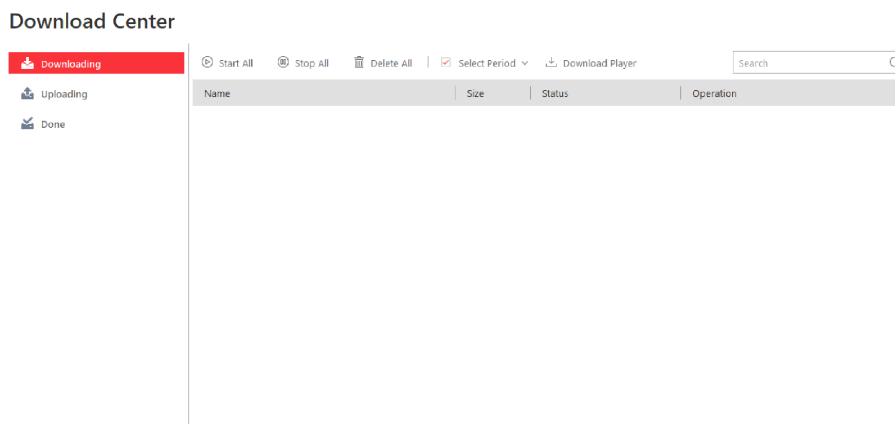
Figure 10-1 Download Center
