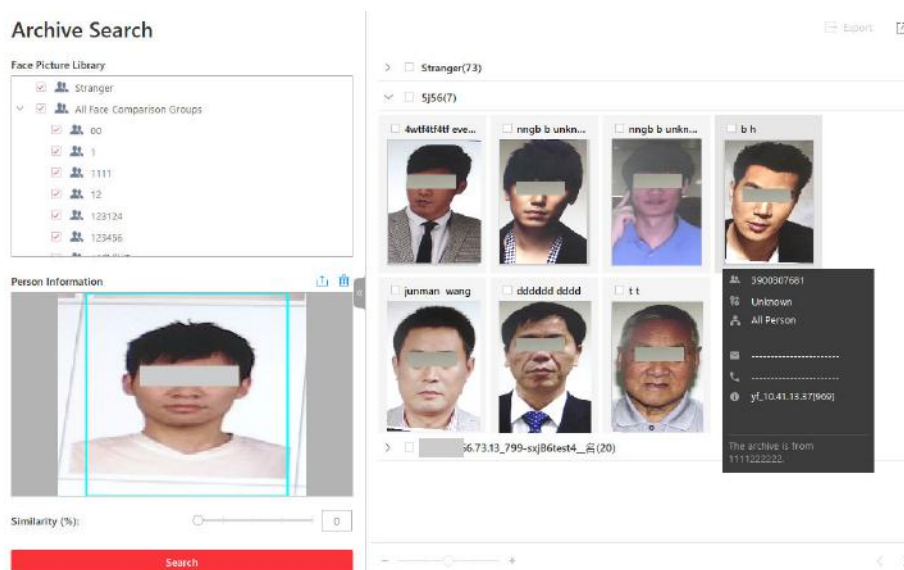
Figure 15-7 Archive Search
