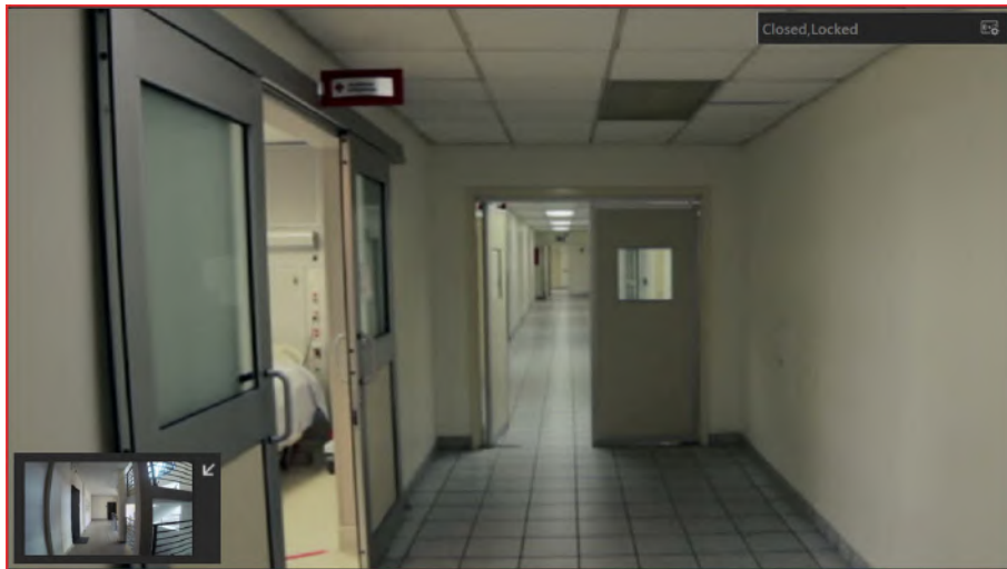
Figure 13-1 Picture-in-Picture Mode
