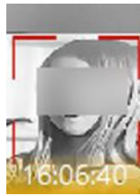
Figure 15-1 Mismatched Person
