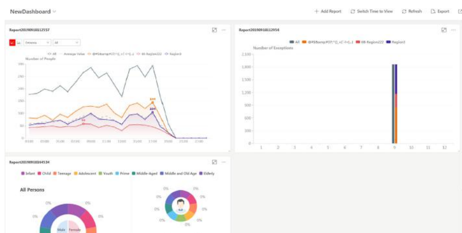
Figure 20-1 Report Dashboard
