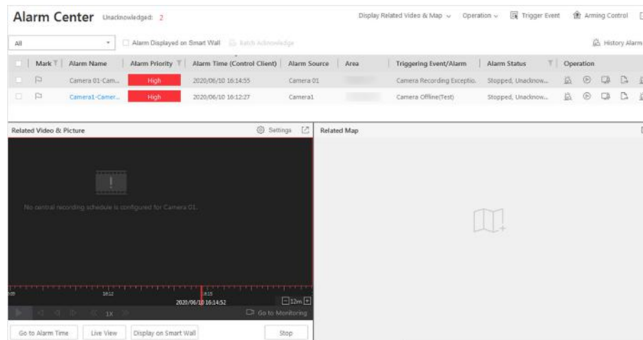
Figure 17-2 Alarm Center
