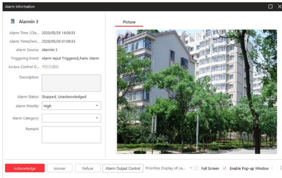
Figure 16-3 Panic Alarm
