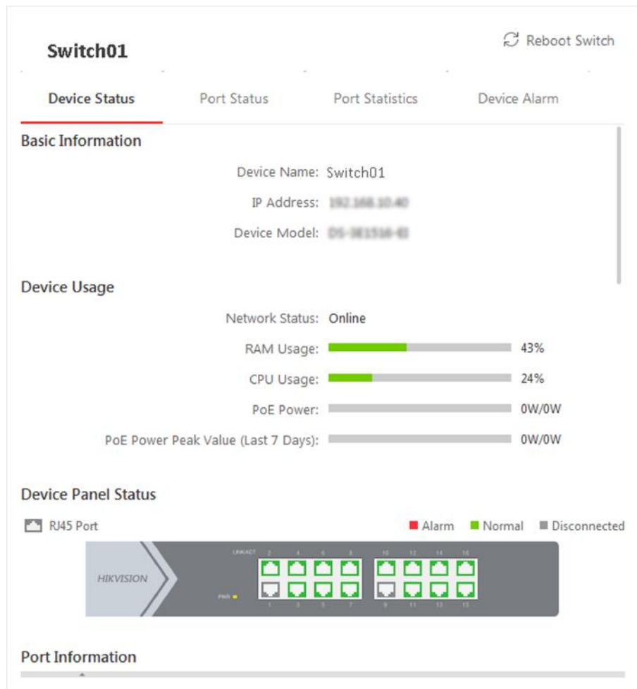
Figure 21-6 Device Details
