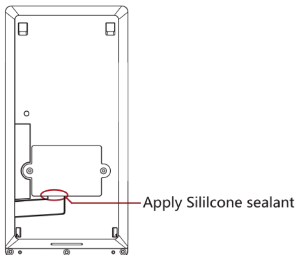
Figure 3-3 Apply Silicone Sealant
