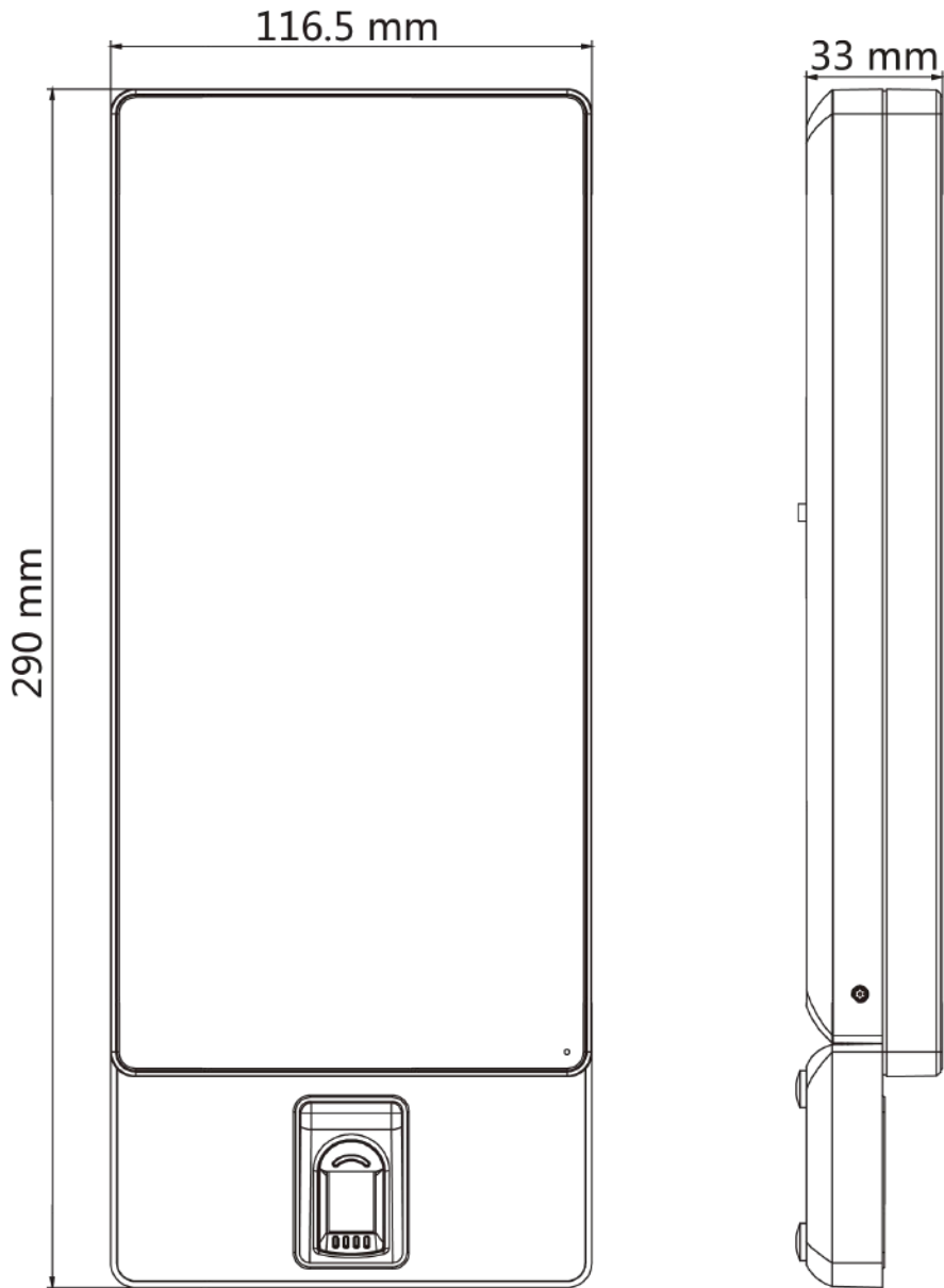
Figure D-1 Device with Fingerprint Module
