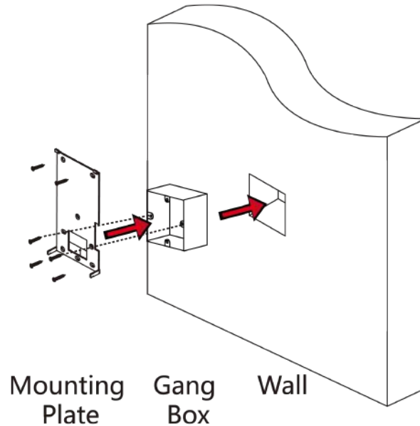
Figure 3-2 Install Mounting Plate
