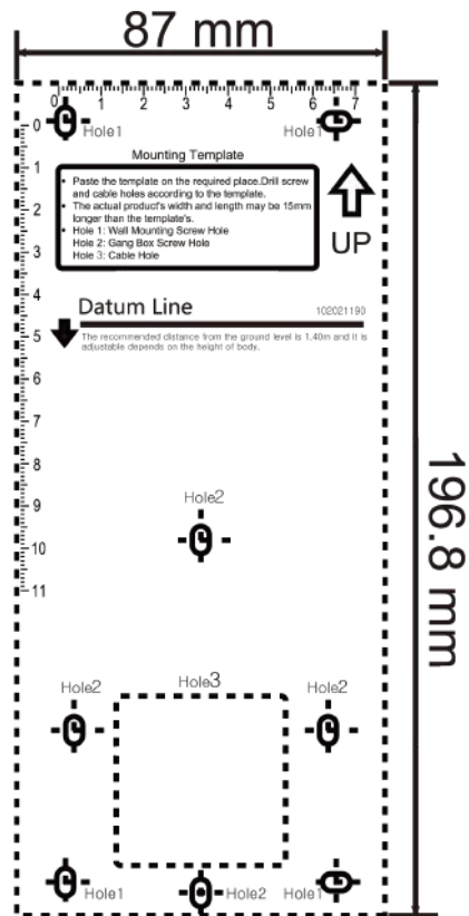
Figure 3-7 Mounting Template
