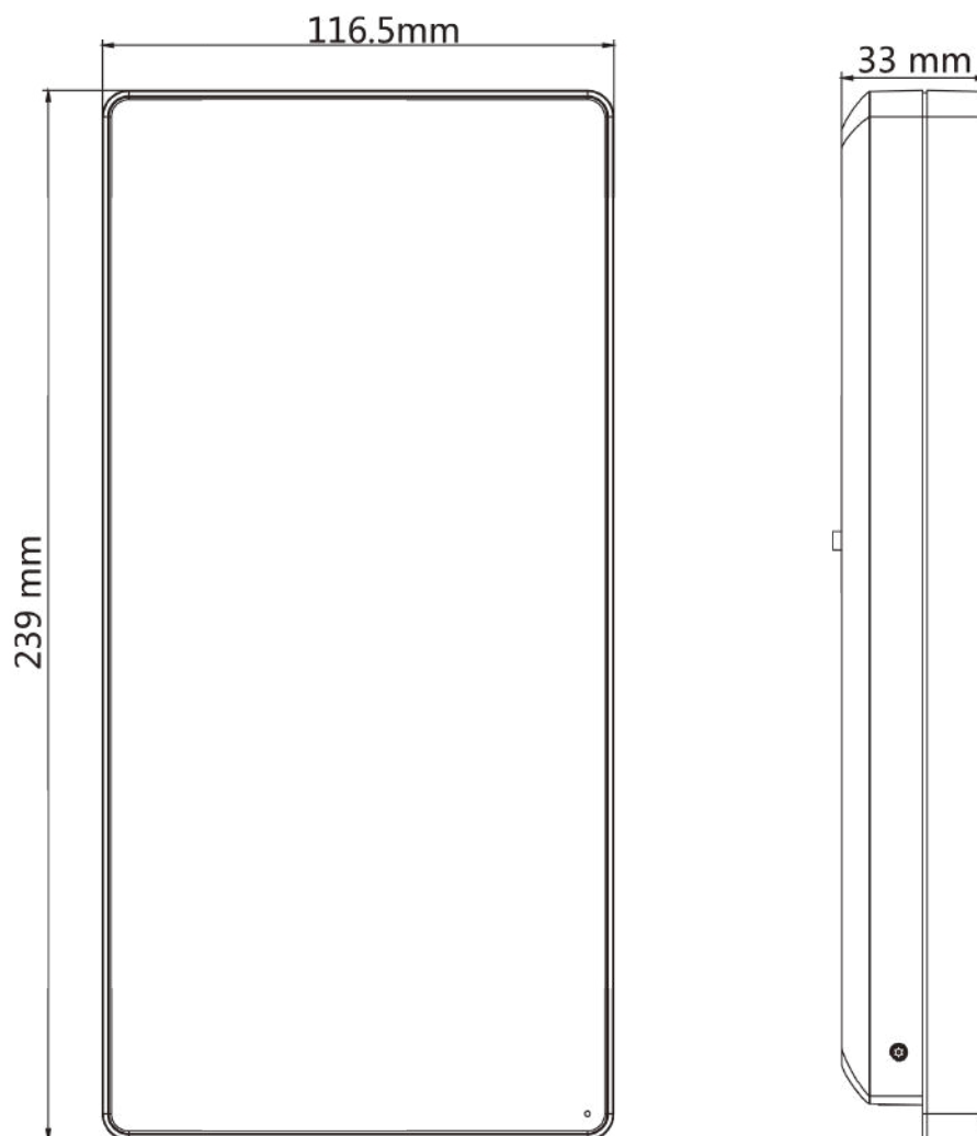
Figure D-2 Device without Fingerprint Module
