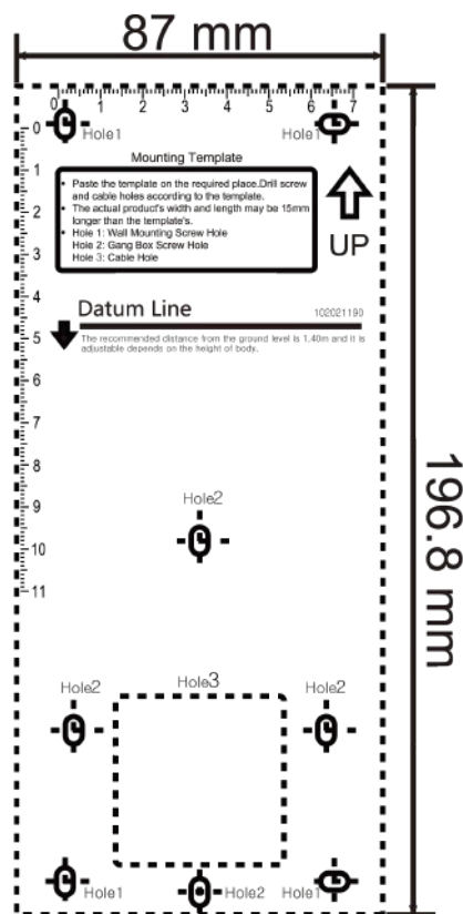
Figure 3-1 Mounting Template
