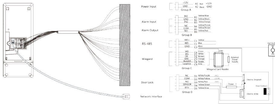
Figure 4-2 Device Wiring
