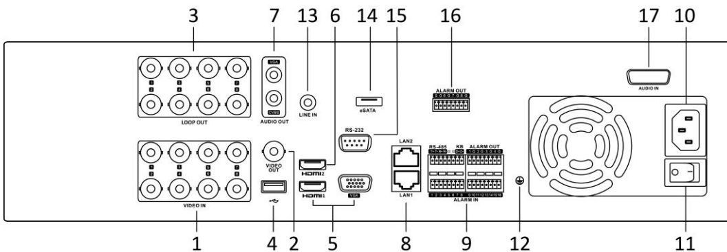
Figure 1-26 Rear Panel of DS-9000HUHI-K8 (with 8 Video Inputs)
