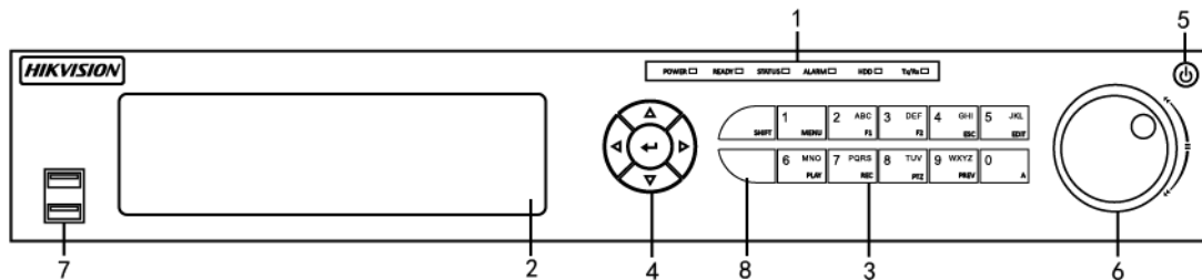
Figure 1-2 Front Panel
